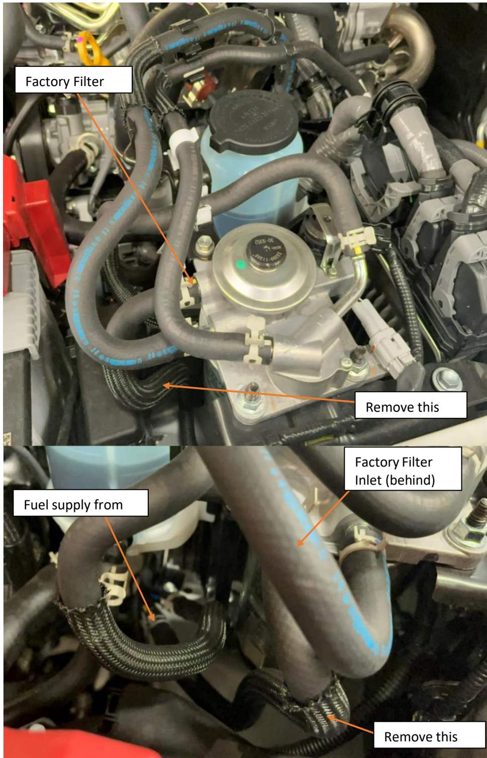
Factory Fuel Filter hose locations
