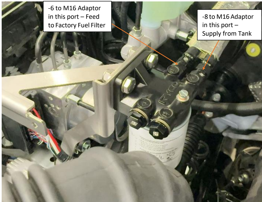
Ryco filter in place on bracket with Adaptors installed.
