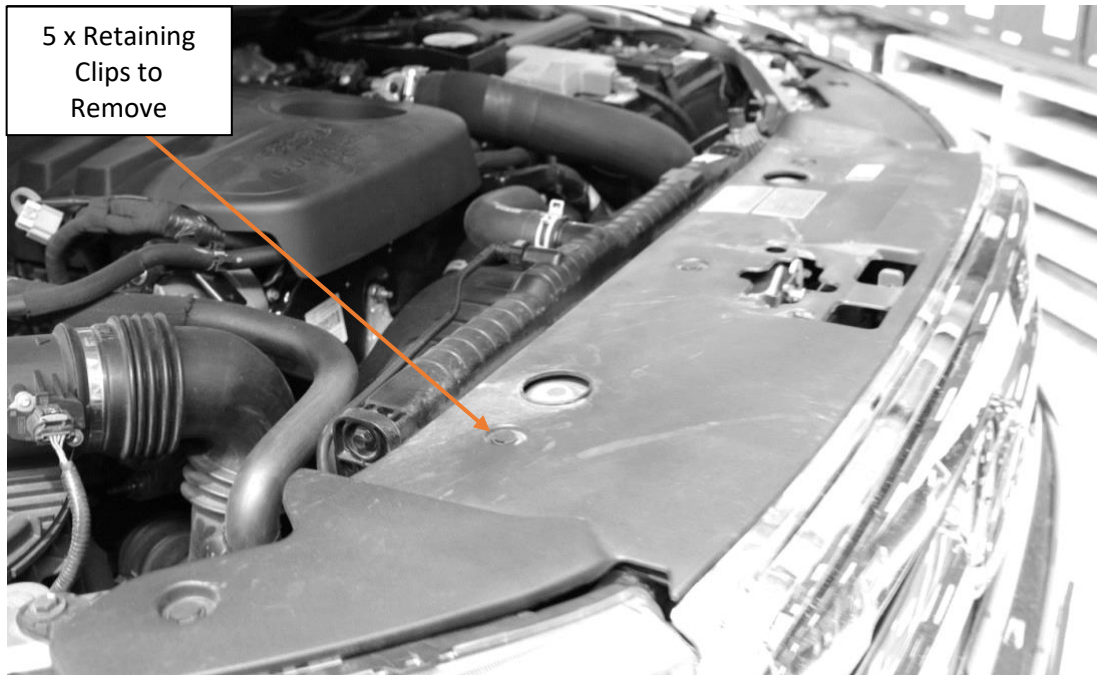
PX2 Ranger Front of Engine Bay
